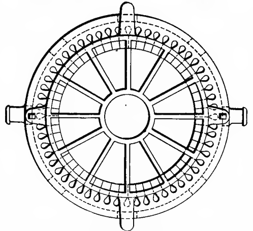
Fig. 5376. Plan. THE WHITNEY CONTRACTING-CHILL.
